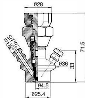
Welded Aseptic Sample Valve No.LV-I003
