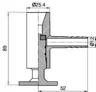
Welded Sample Valve
