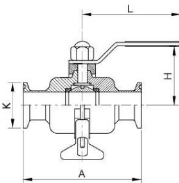
Clamped Non-retention Ball Valve
