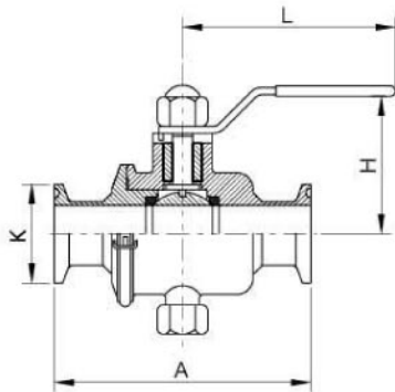
Clamped Portable Ball Valve
