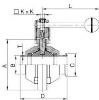
Welded / Clamped Butterfly-type Ball Valve
