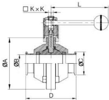
Clamped Butterfly-type Ball Valve
