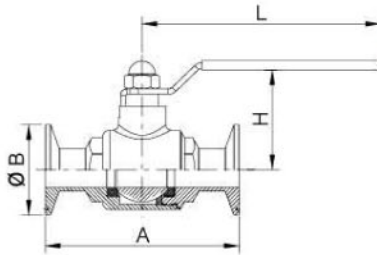
Clamped Straight Ball Valve
