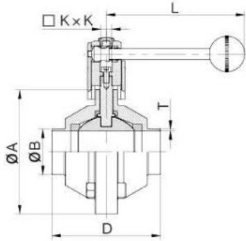
Welded Butterfly-type Ball Valve
